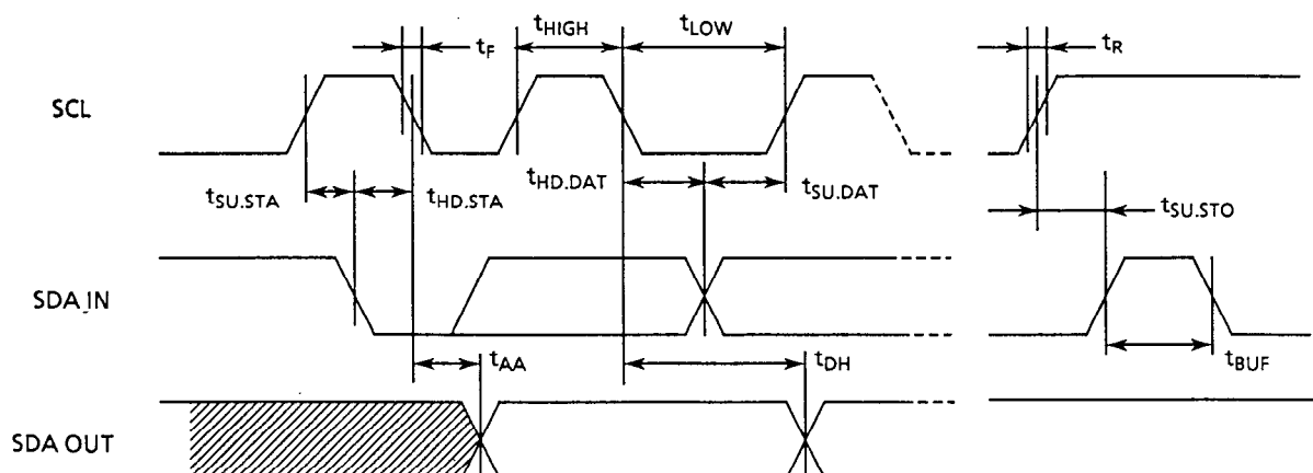
Figure 4 Bus Timing
